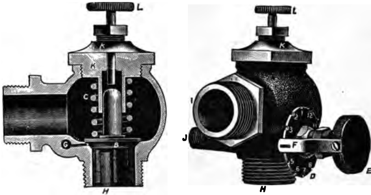
FIG. 165.—The James-Lunkenheimer Improved Mixing Valve. B, fuel inlet valve; C, spring controlling B; E, the wheel controlling gasoline valve; F, clip or top for holding E in position; G, gasoline supply tube; H, air inlet; I, entrance to cylinder; J, entrance for gasoline; K, cover of valve chamber; wheel and spindle controlling tension of spring, C.
